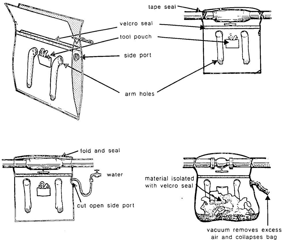
FIGURE 4 USE OF GLOVE BAGS
