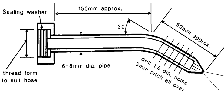
FIGURE 3 TOTAL SATURATION INJECTION HEAD
