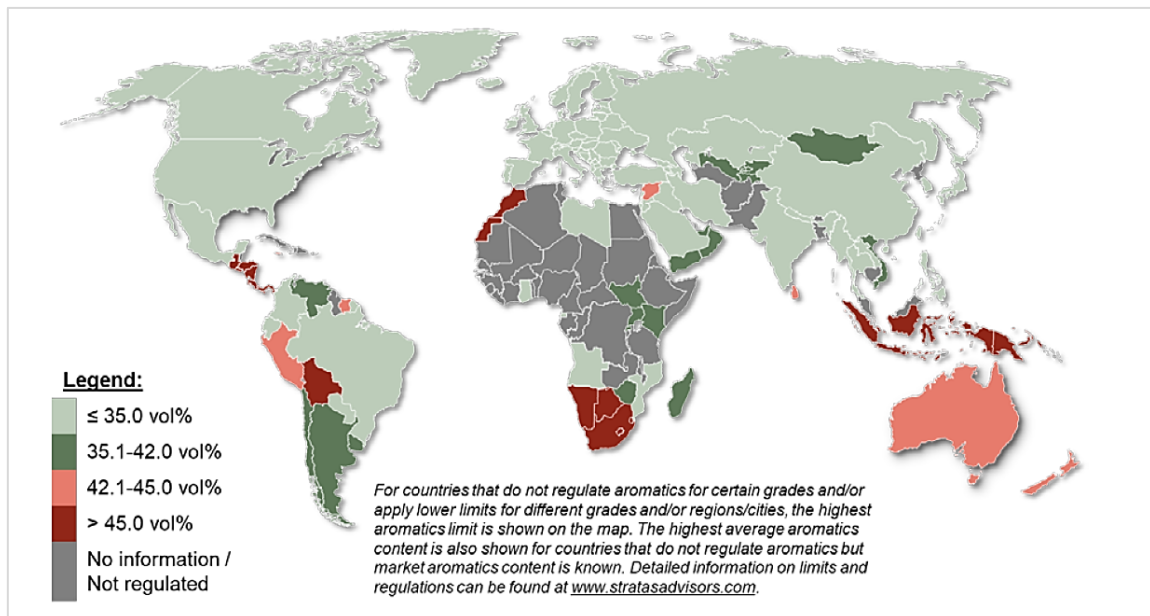
Figure 4: Maximum aromatics content in petrol per country – 2021
