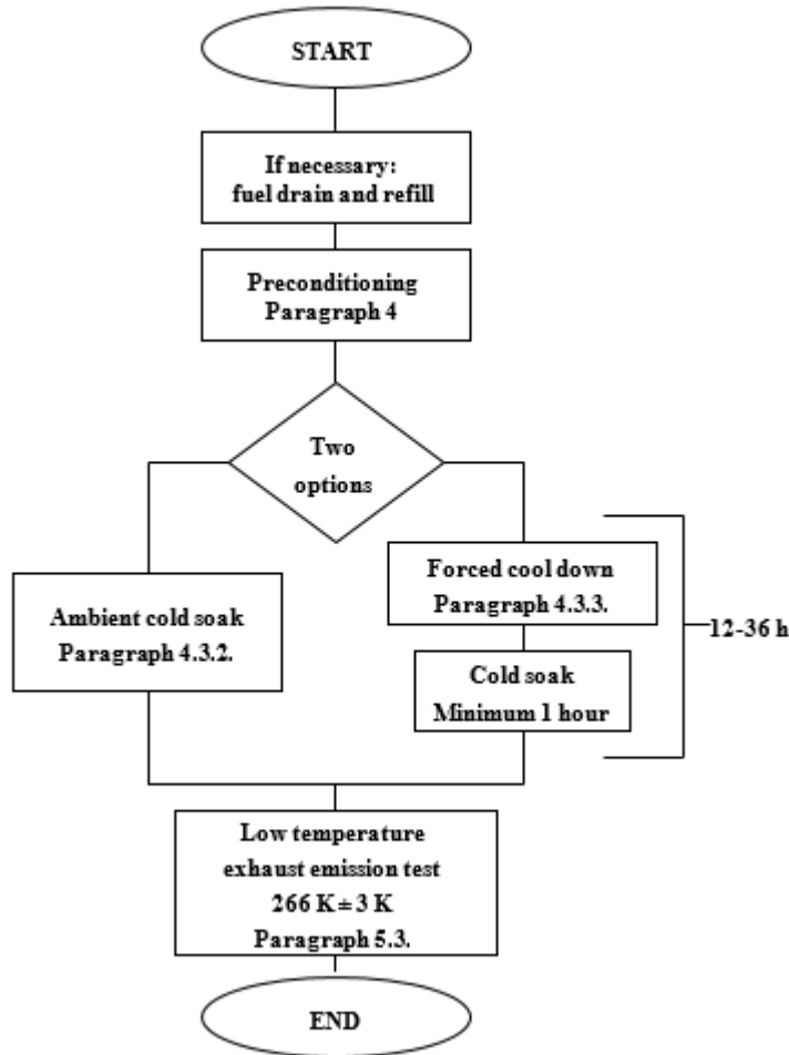
Figure A8/1 Procedure for low ambient temperature test
