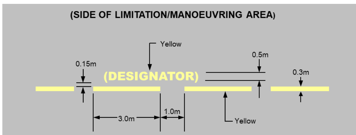
Figure 8.51 (2) Apron limit line with optional designator (shows matters)
