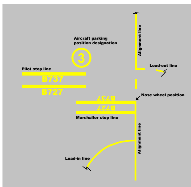
Figure 8.58 (2)-2 Aircraft parking position markings (illustrates matters)
