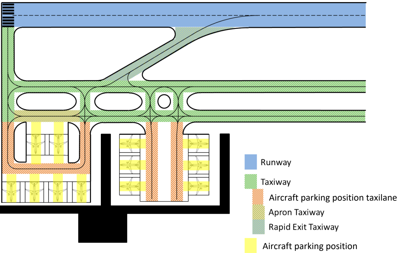
Figure Division 2 Taxiways (illustrates matters)
