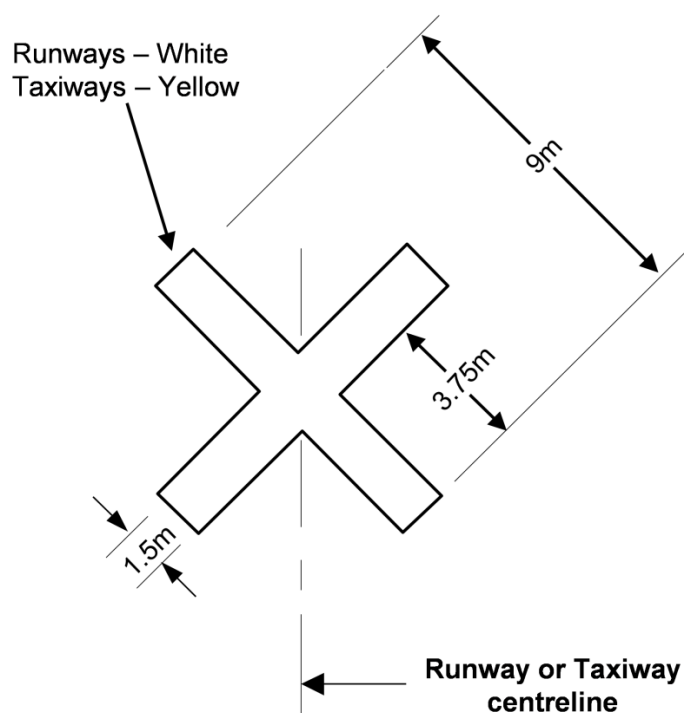
Figure 8.106 (9)-1 Unserviceability marking — temporary closures for runways of 18\text{ m} < \text{width} \leq 30\text{ m} and taxiways, and for permanent closures of all taxiways (shows matters)
