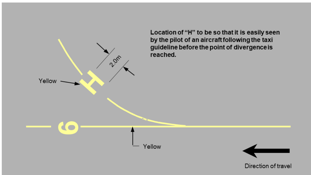
Figure 8.121 (3) Helicopter taxi guideline designator to a single helicopter parking position (prefix only) (shows matters)
