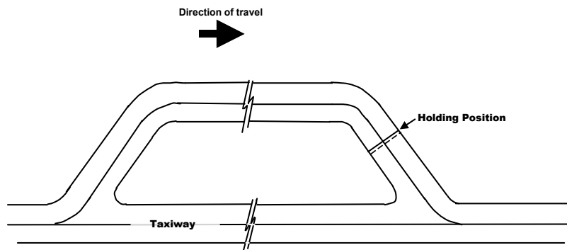
Figure 8.44 (2) Holding bay markings (illustrates matters)
