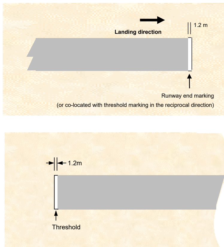
Figure 8.20 (1) Runway end markings (shows matters)
