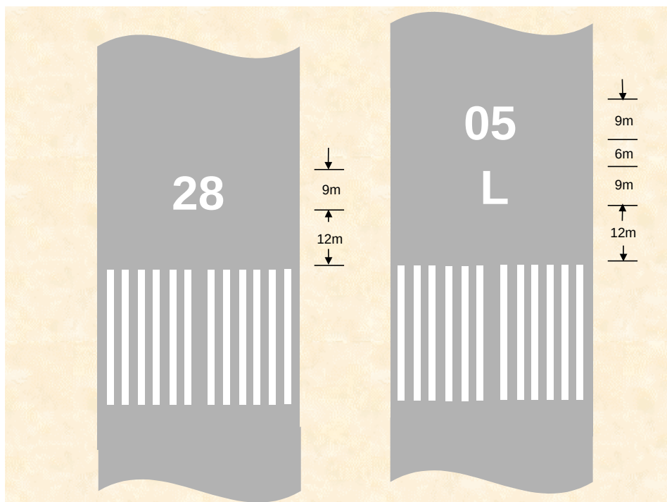
Figure 8.18 (6) Runway design markings (shows matters)
