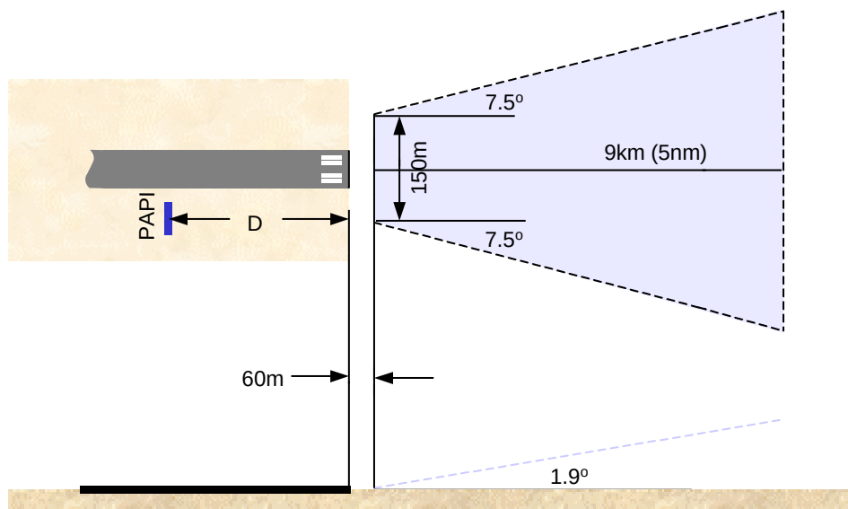
Figure 9.45 (1) Obstacle assessment surface for 3^\circ approach slope (illustrates matters)
