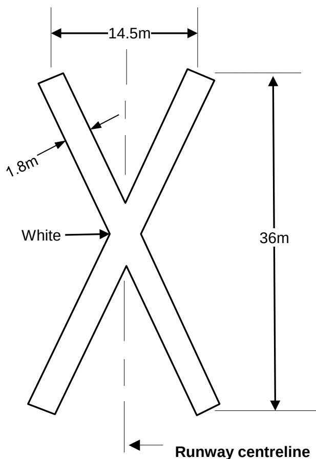
Figure 8.106 (8) Unserviceability marking — temporary closures for runways of width > 30\text{ m} and for permanent closures of all runway widths (shows matters)
