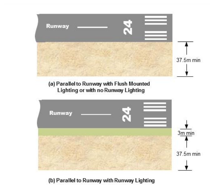
Figure 6.66 (3) Glider runway strip (illustrates matters)
