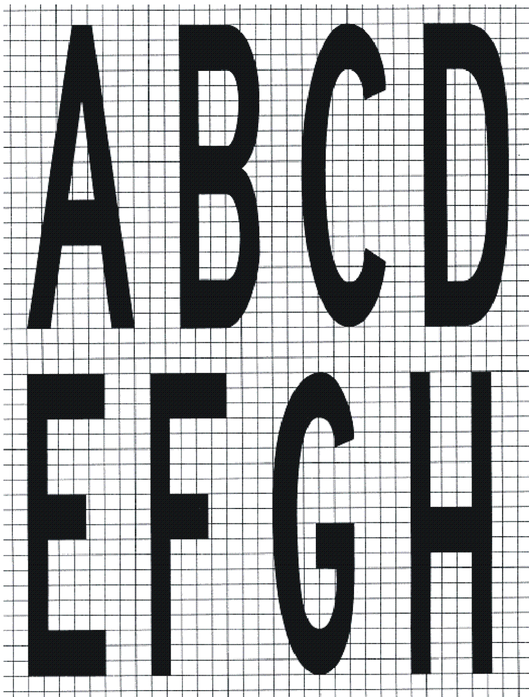
Figure 8.69 (1)-1 Letters and numbers used in designations for taxiway and apron markings (shows matters)
