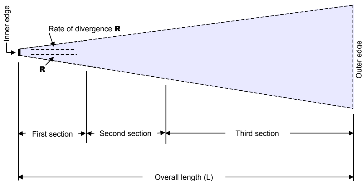
Figure 7.08 (6)-2 Plane view of approach surface
