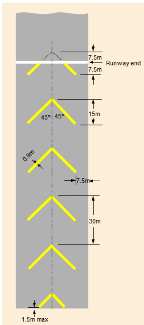
Figure 8.16 (2) Pre-threshold area markings (shows matters)
