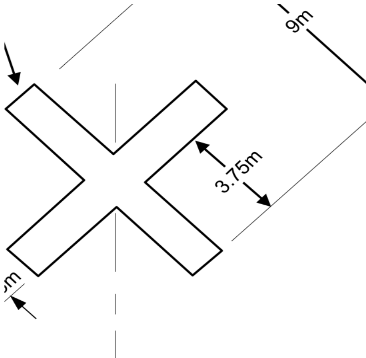
Figure 8.106 (9)-1 Unserviceability marking — temporary closures for runways of 18\text{ m} < \text{width} \leq 30\text{ m} and taxiways, and for permanent closures of all taxiways (shows matters)
