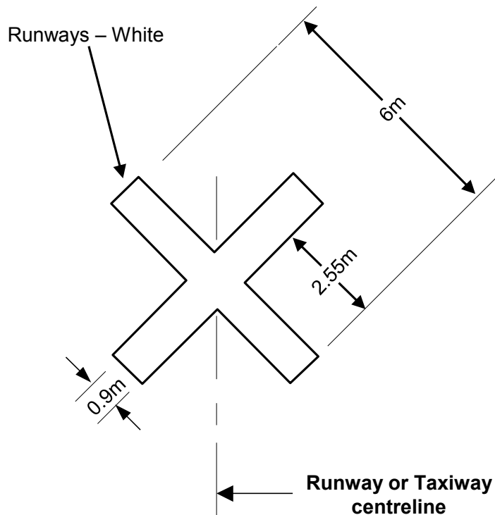
Figure 8.106 (9)-2 Unserviceability marking — temporary closures for runways of 18\text{ m} width (shows matters)
