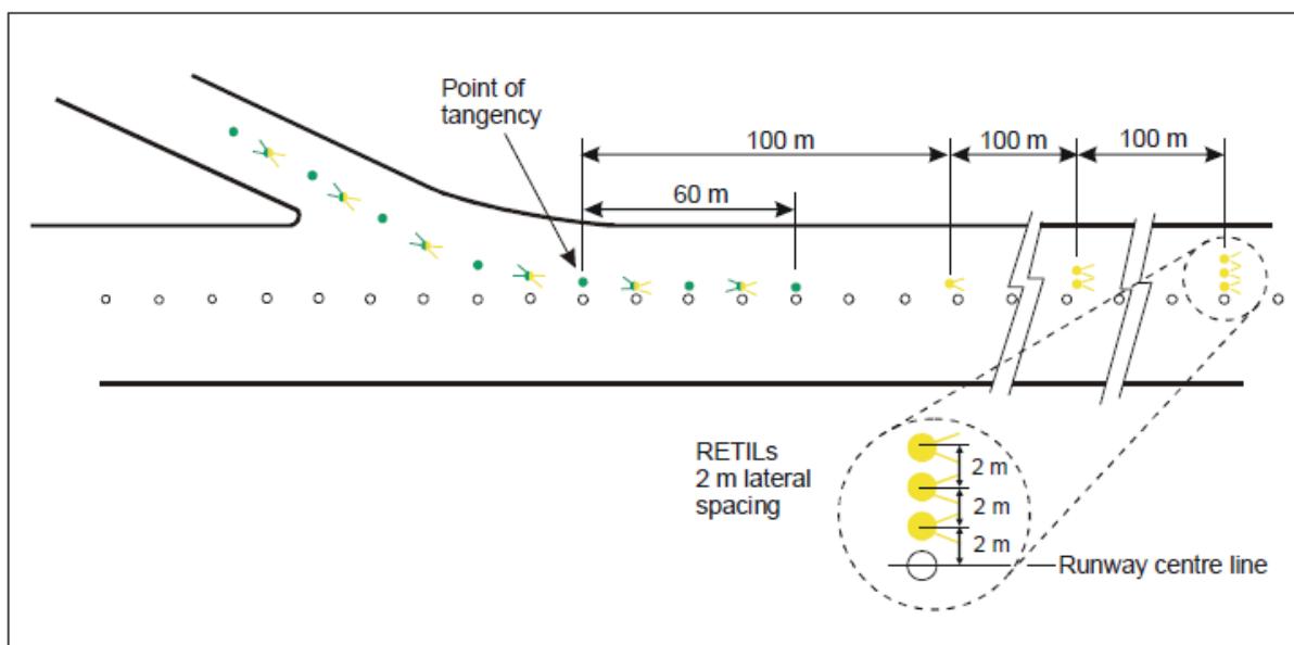
Figure 9.89 (2) Rapid exit taxiway indicator lights (shows matters)
