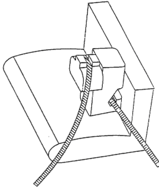
FIGURE 2 INSTALLATION OF FIXTURE ONTO VEHICLE SEAT (see paragraph 2.6.1.)
