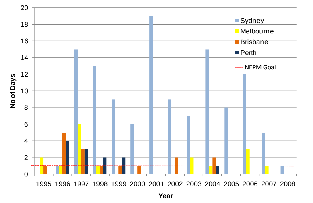
Figure A1 Number of Days NEPM 1hr Ozone Standard (0.10ppm) Exceeded in Four Australian Cities
