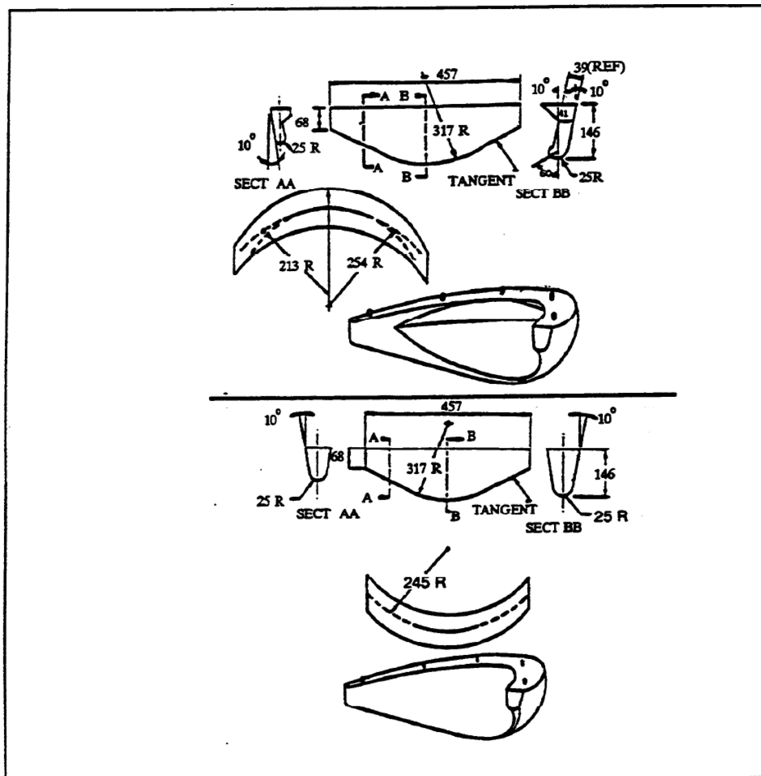
Figure 2 - Diagrams of 'Bead' Unseating Blocks (dimensions in mm)
