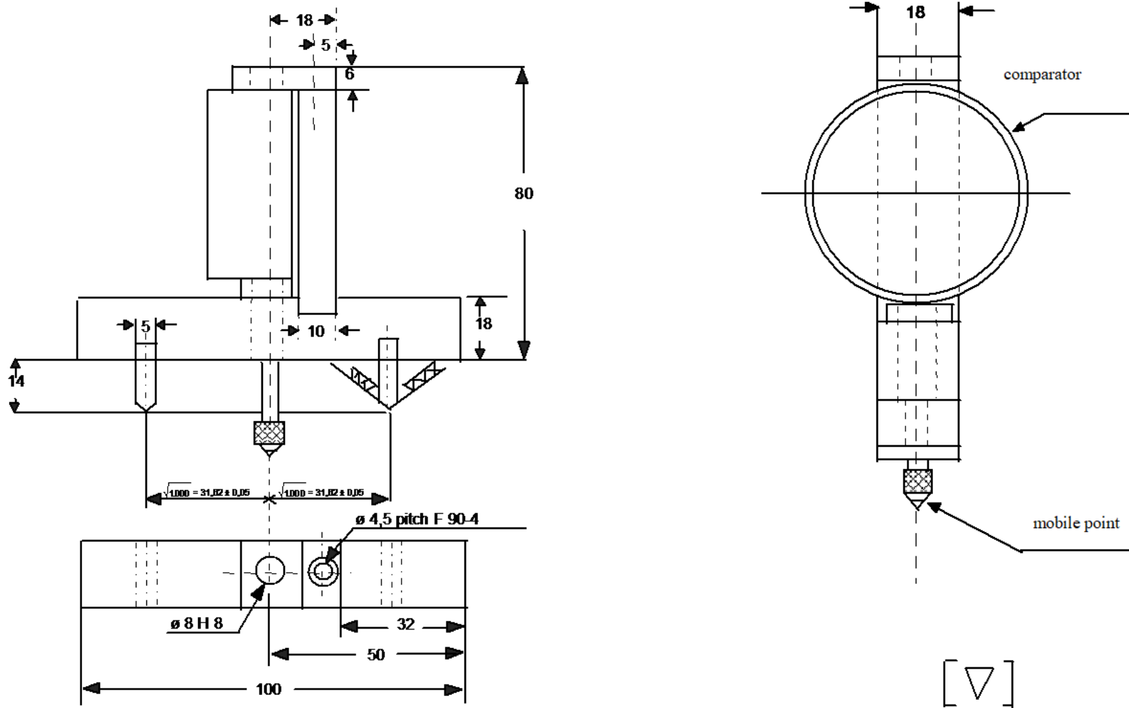
Figure 1: Spherometer
