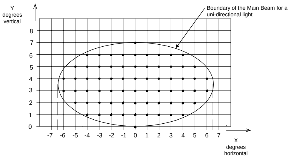
Figure 9.11-12: Method of Establishing Grid Points to be used for the Calculation of Average Intensity of Runway Lights specified by Figure 9.11-1 to Figure 9.11-10
