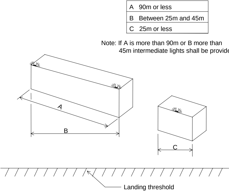
Figure 9.4-3: Typical lighting of horizontally extended obstructions
