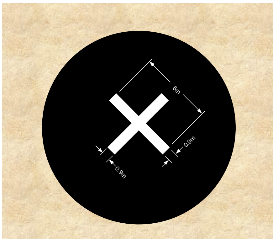
Figure 13.1-5: Total unserviceability marking
