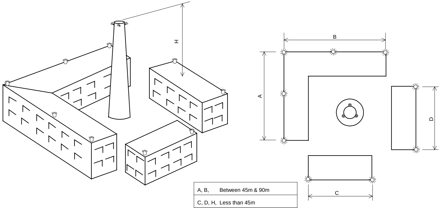
Figure 9.4-2: Typical lighting of a group of obstructions
