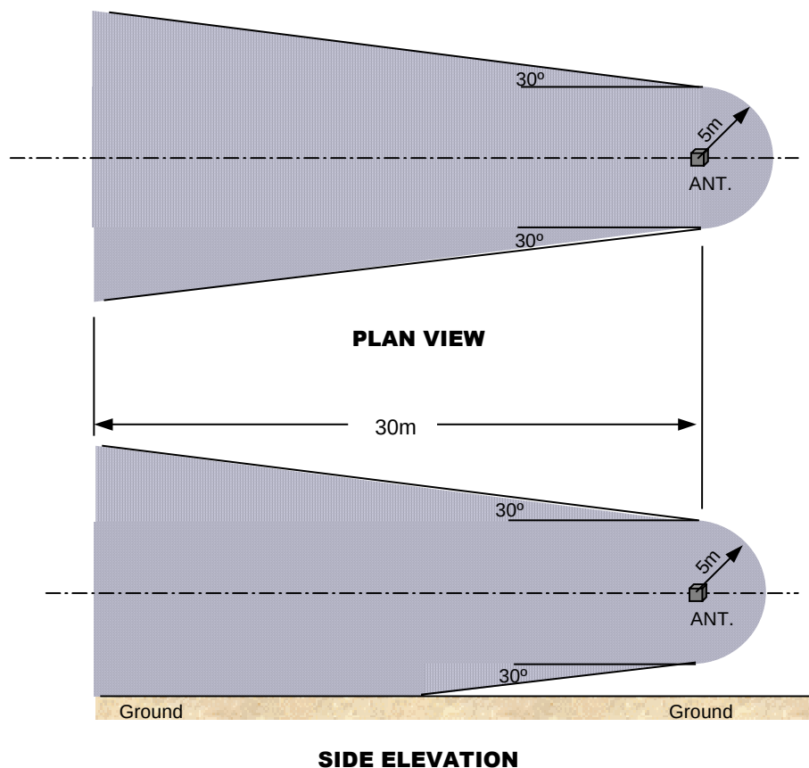
Figure 11.1-3: ILS Remote monitor antenna sensitive area
