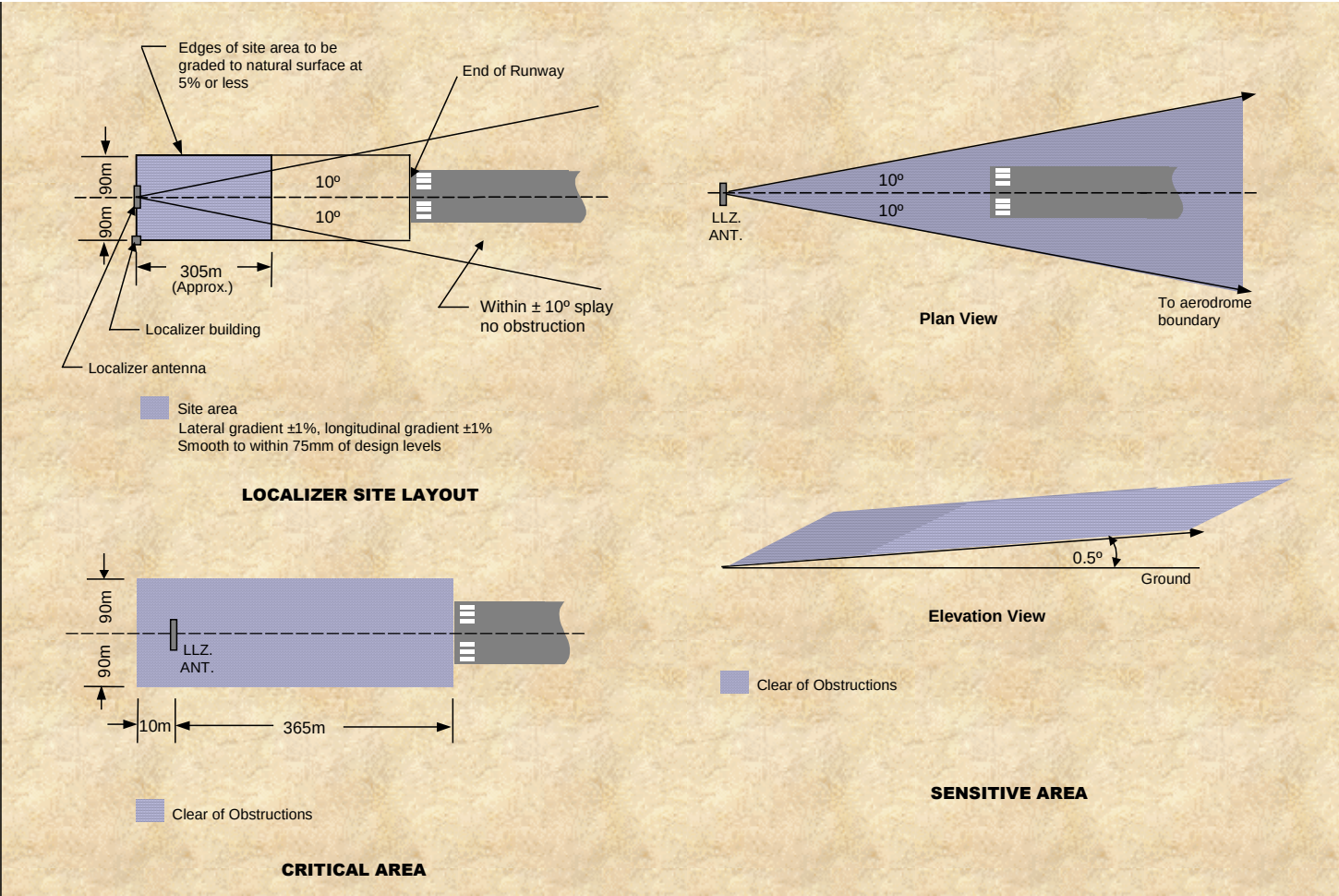
Figure 11.1-1: ILS localizer site preparation and restrictions
