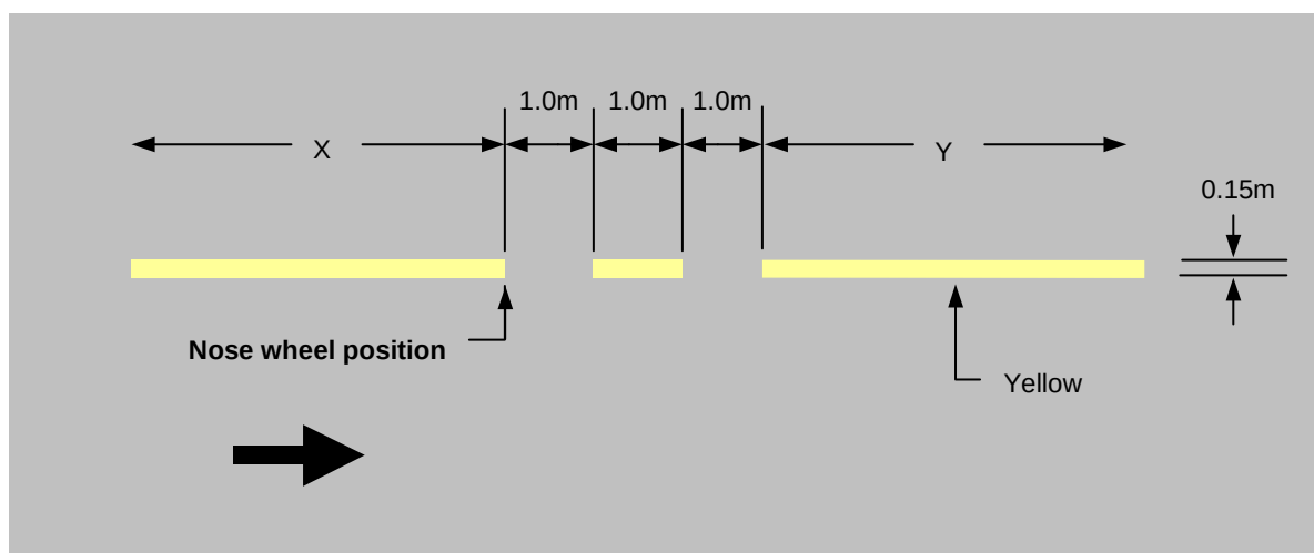
Figure 8.5-13: Alignment line
