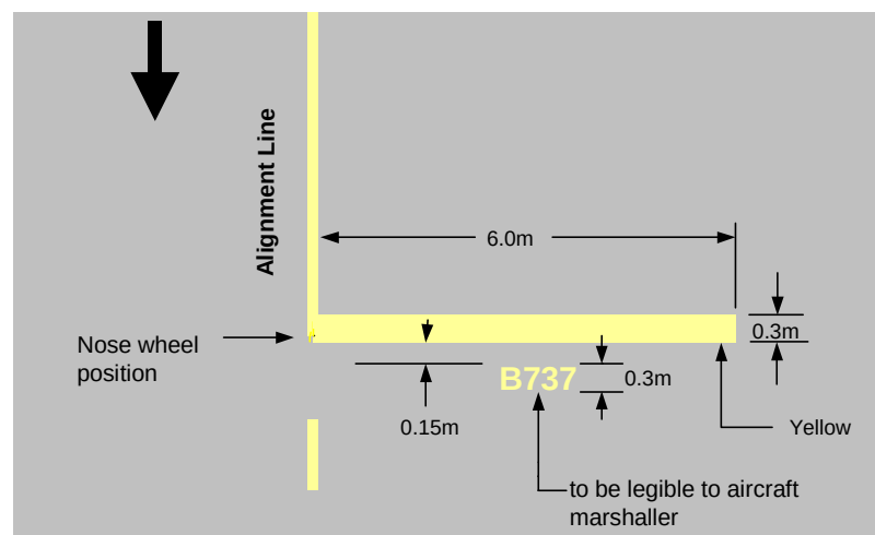
Figure 8.5-11: Marshaller stop line
