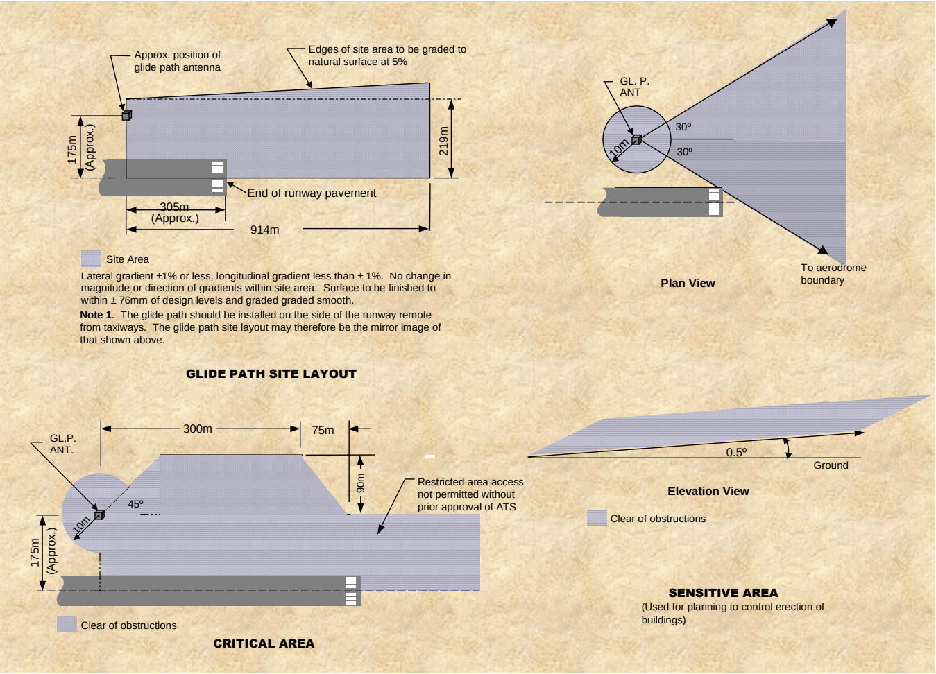
Figure 11.1-2: ILS Glide path site preparation and restrictions
