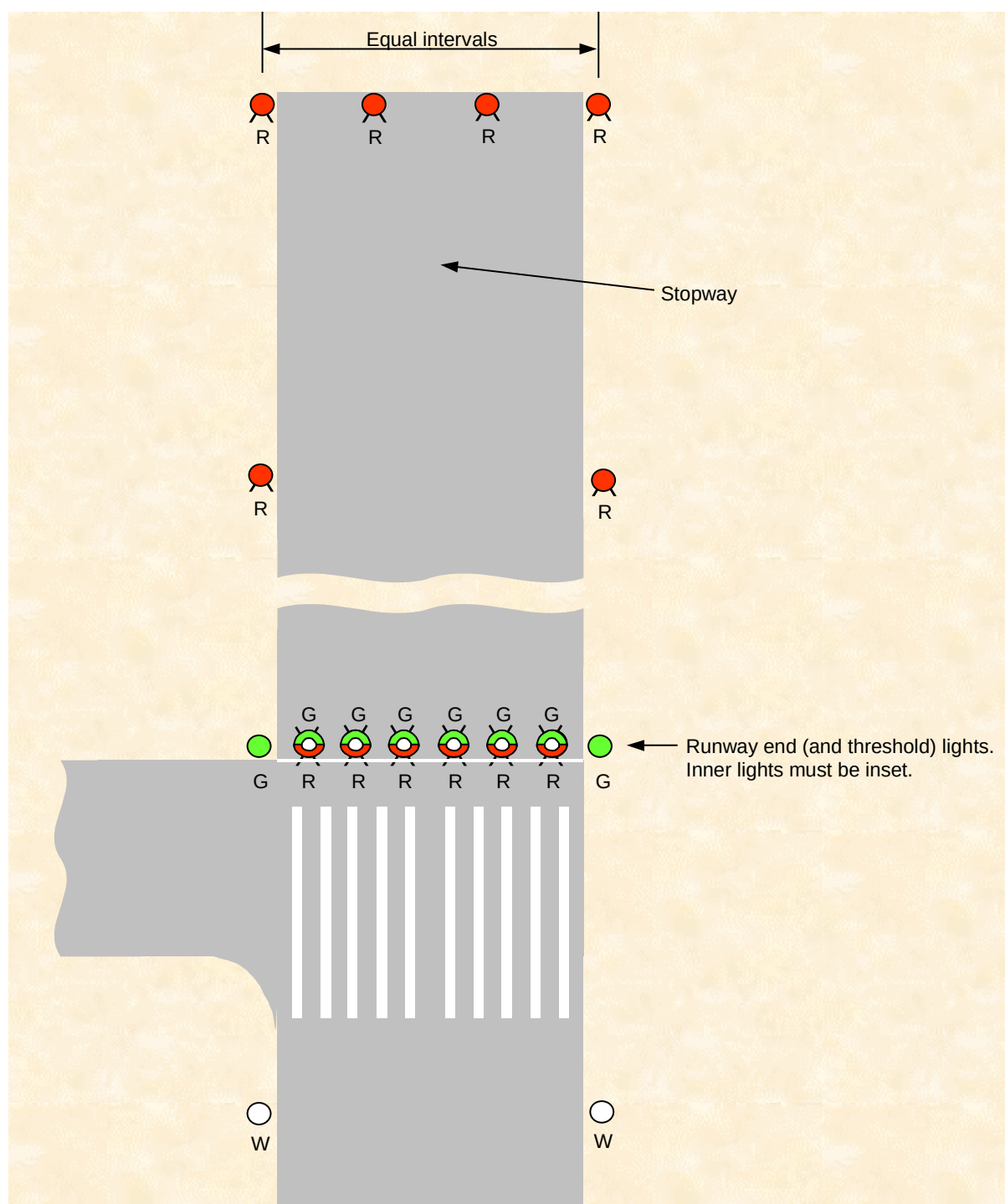
Figure 9.12-5: Typical Stopway Lights
