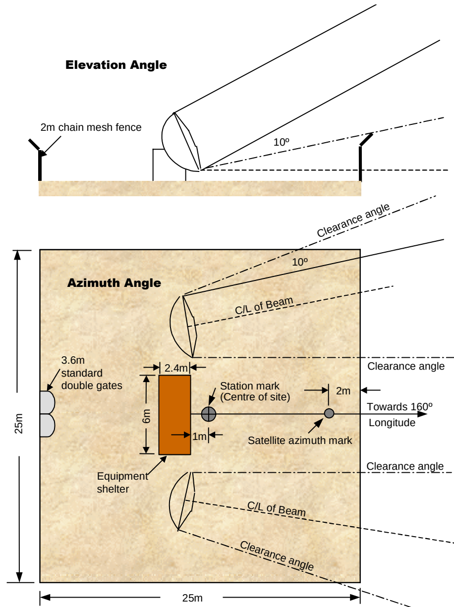
Figure 11.1-4: Communications Satellite Ground Station Manned Centre Site
