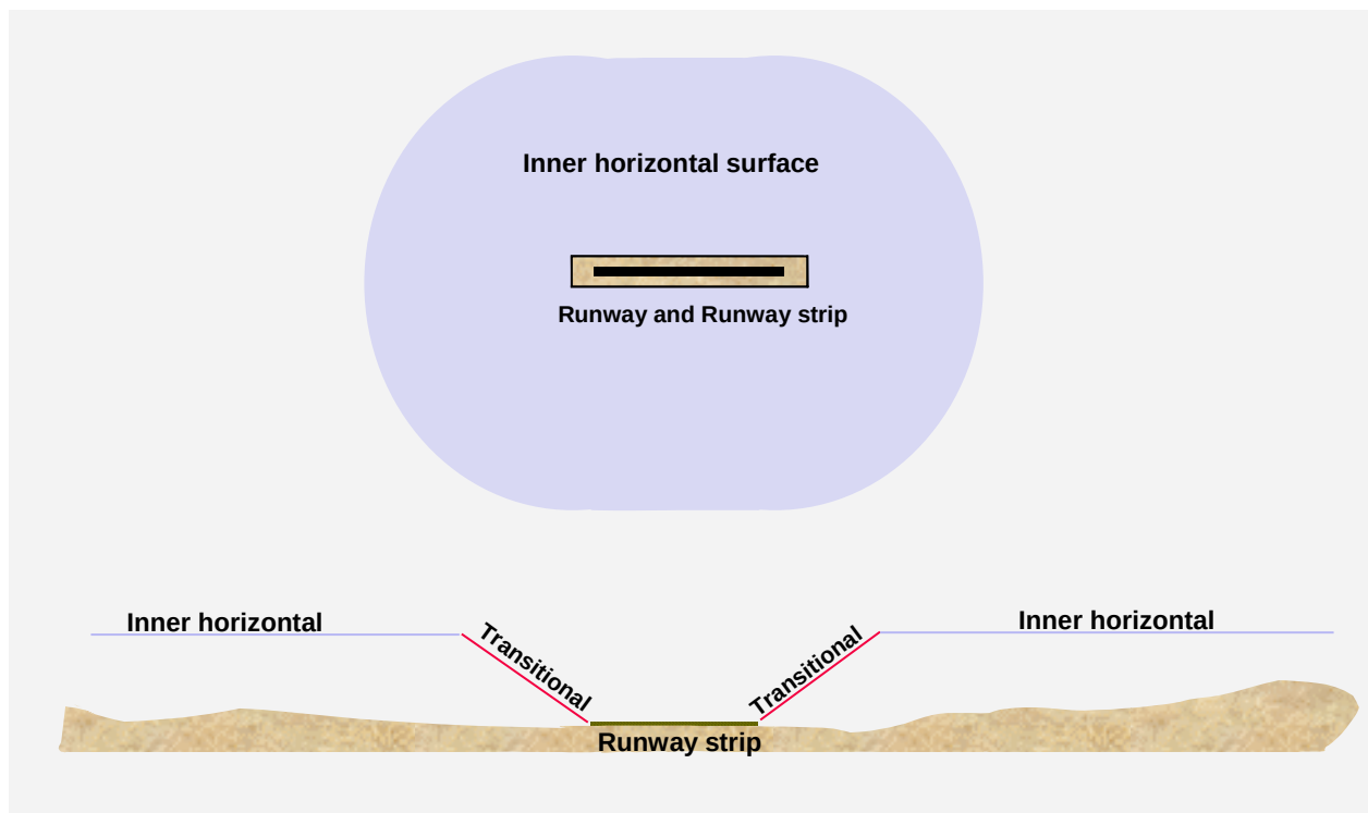
Figure 13.1-2: OLS cross-section
