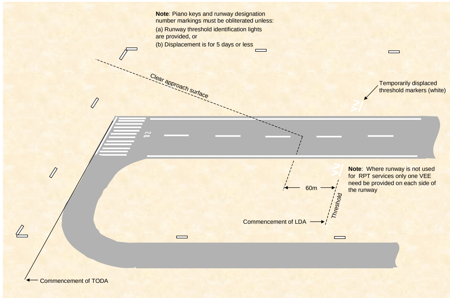
Figure 8.3-15: Markings for a temporarily displaced threshold due to obstacle infringement of approach surface for a period of 5 days or less and a displacement of less than 450 m
