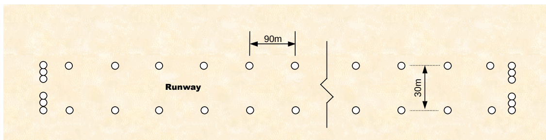
Figure 13.1-4: Aerodrome lighting
