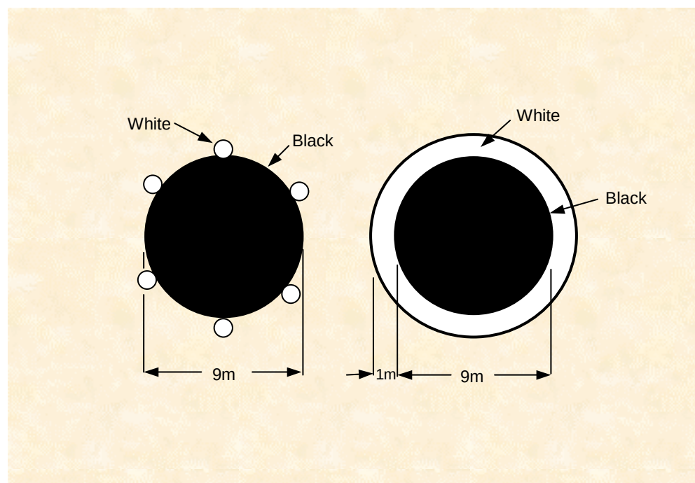
Figure 8.8-1: Signal Area
