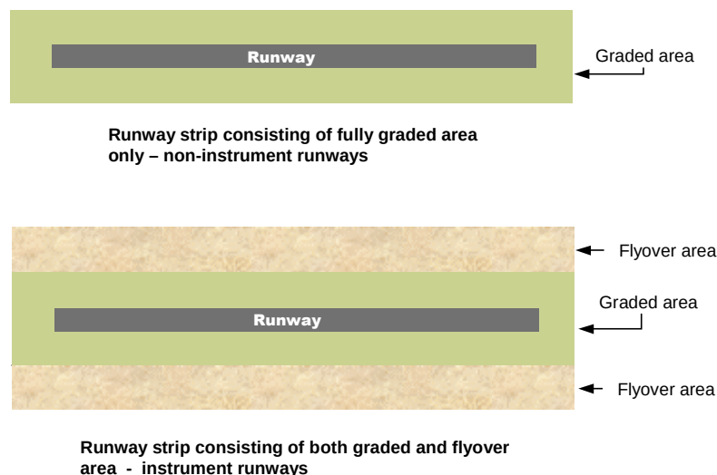
Figure 6.2-2: Composition of Runway Strip
