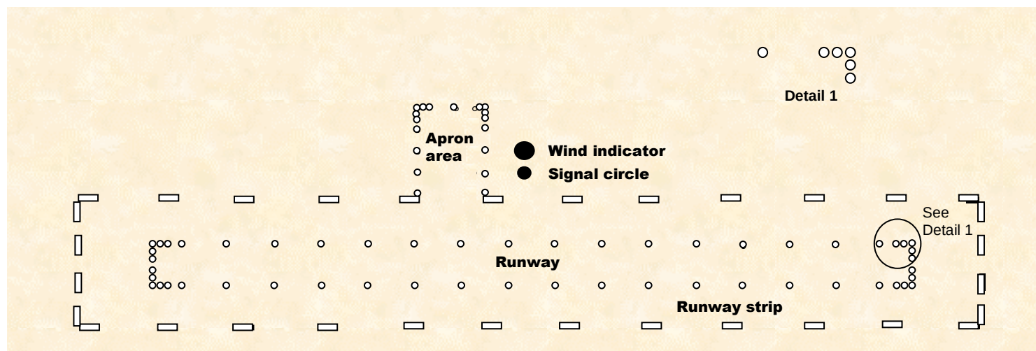
Figure 13.1-3: Aerodrome markings
