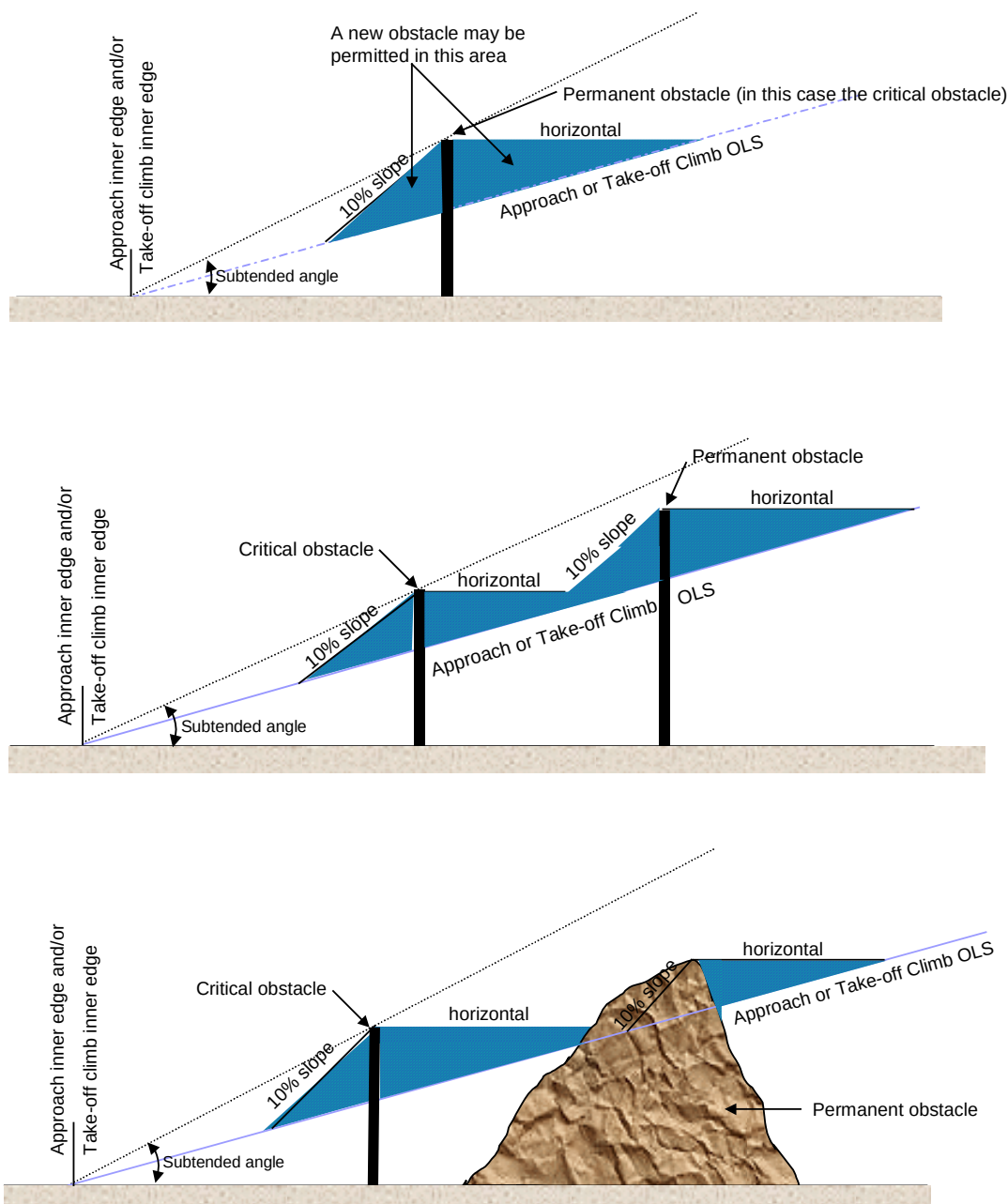
Figure 7.4-1: Shielding of obstacles penetrating the approach and take-off climb surfaces
