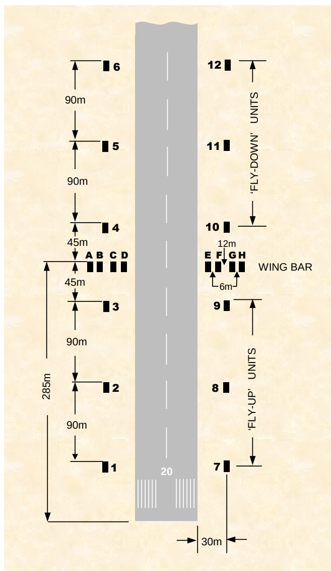
Figure 9.9-2: T-VASIS Layout
