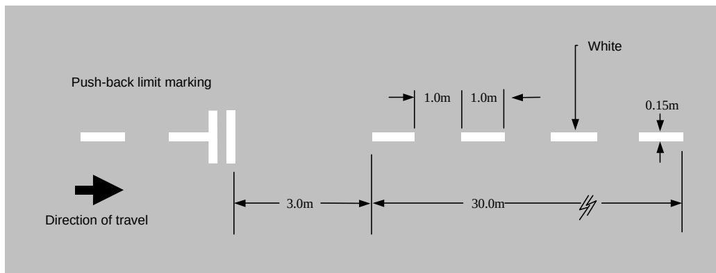
Figure 8.5-27: Push-back alignment line
