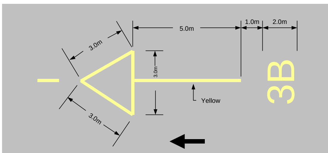
Figure 8.5-15: Triangle marking
