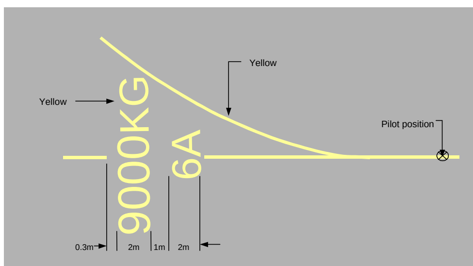
Figure 8.5-10: Aircraft upper weight limit designation
