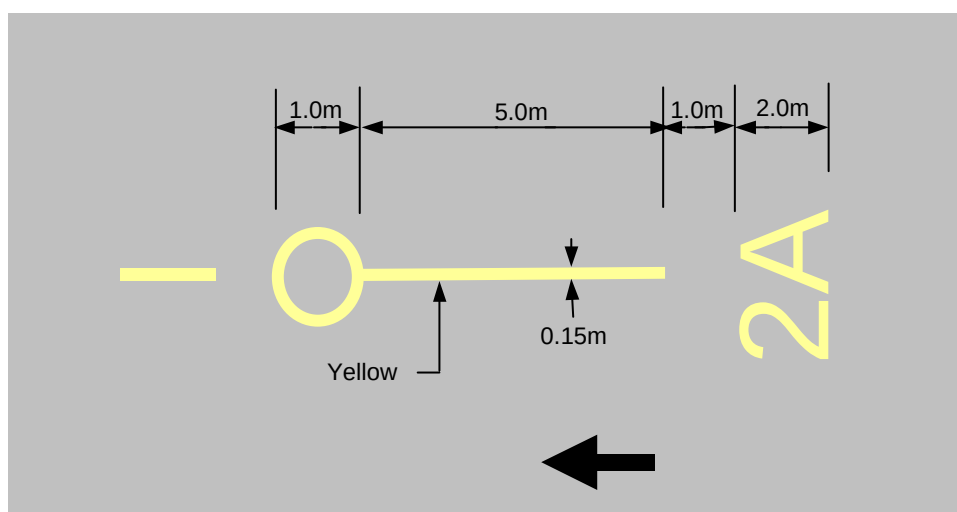
Figure 8.5-14: Keyhole marking
