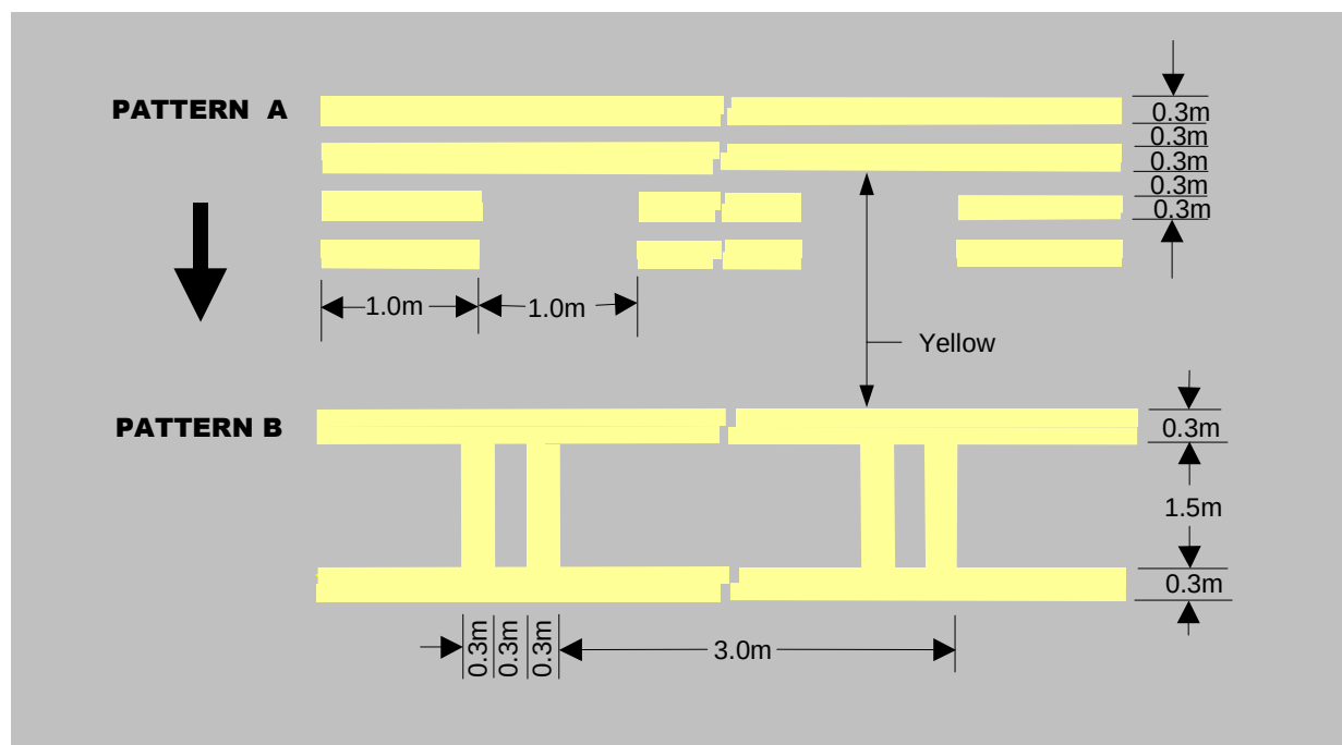
Figure 8.4-3: Pattern A and Pattern B runway-holding position markings — increased conspicuity
