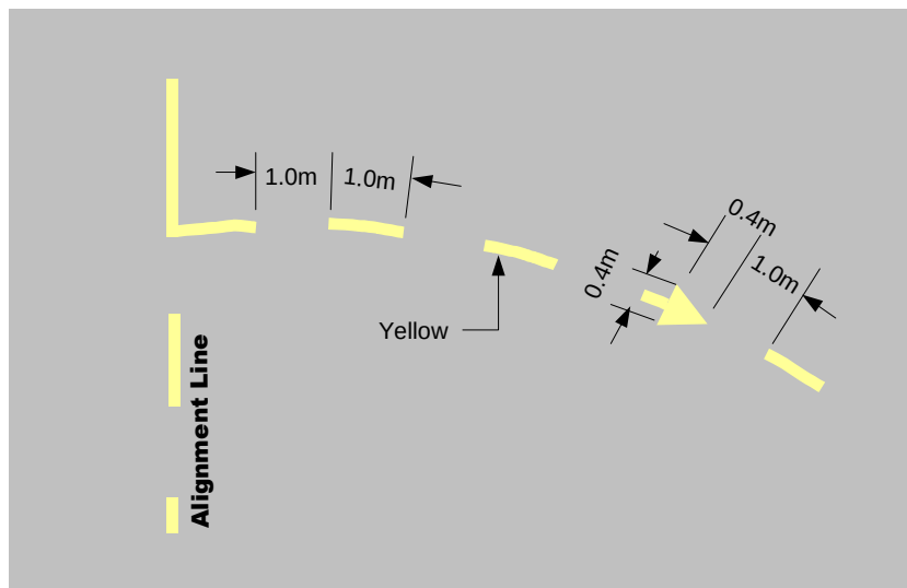
Figure 8.5-16: Lead-out line
