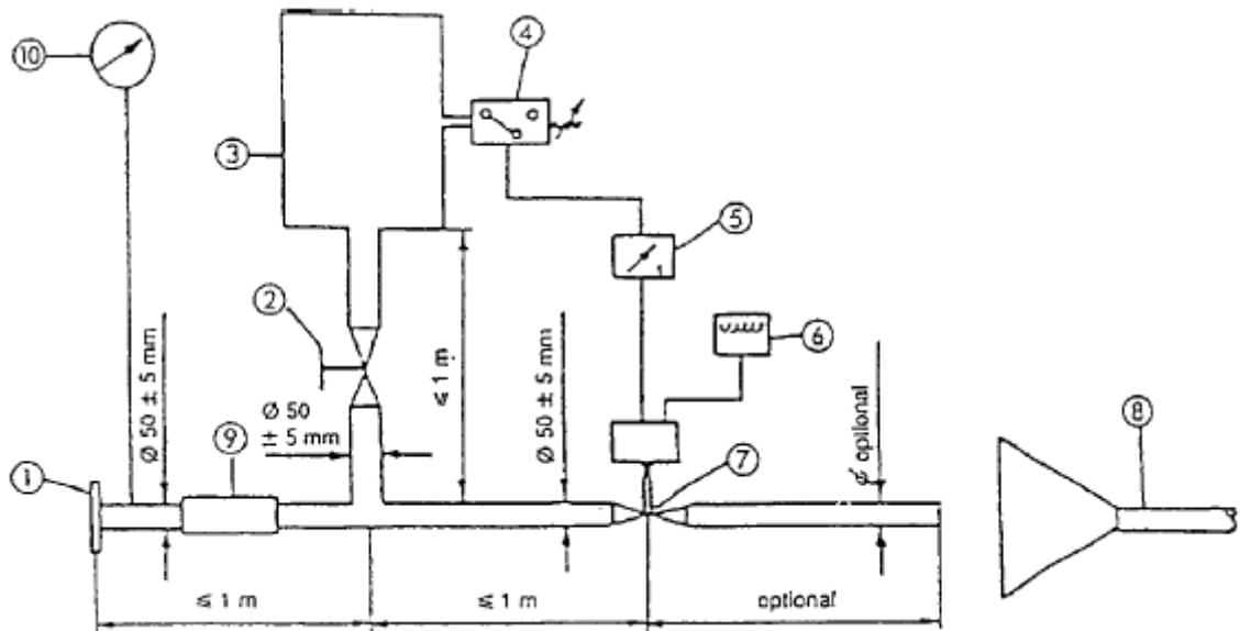
Figure 3. Test apparatus for conditioning by pulsation
