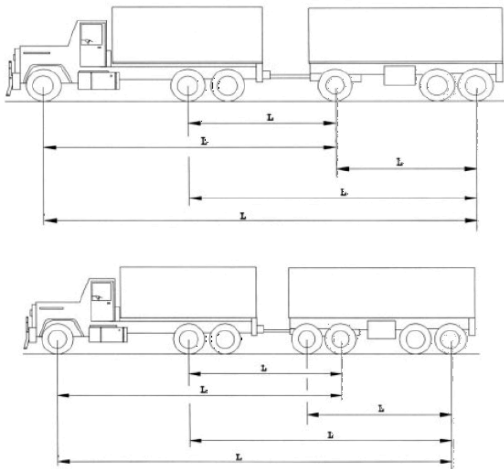
Figure#1 Examples of the calculation of minimum axle group spacing
